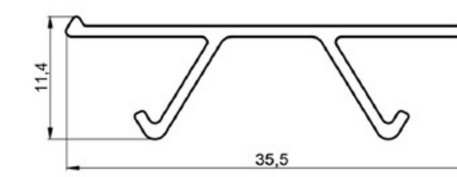
PARTITION BUMPER
