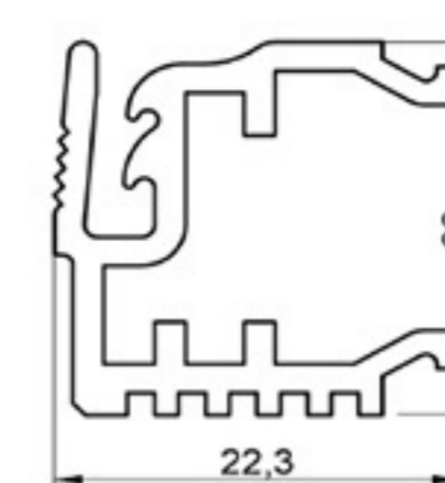
FLOORING LEVELING PROFILE
