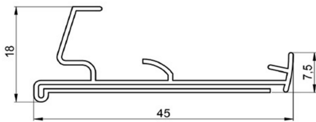
PARTITION BUMPER
