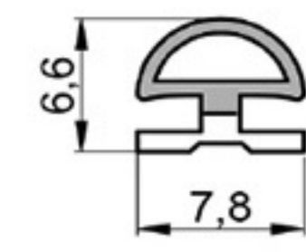
PROFILE FOR PARTITIONS
