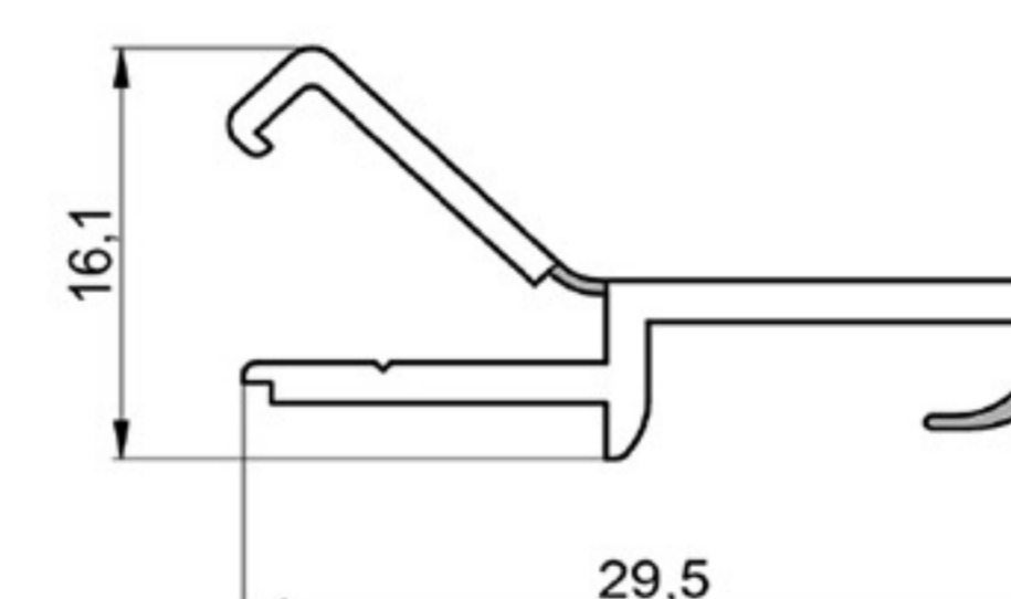
FURNITURE FRAME STOPPER
