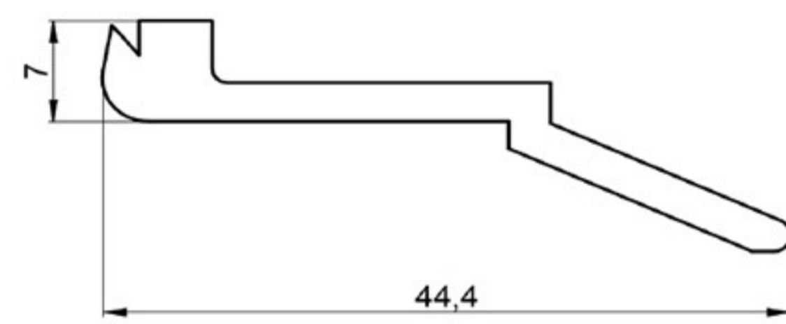
PROFILE FOR PARTITIONS
