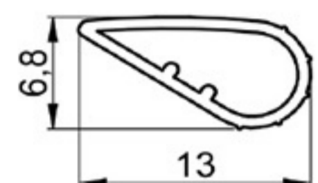
LIGHTING COVER PROFILE
