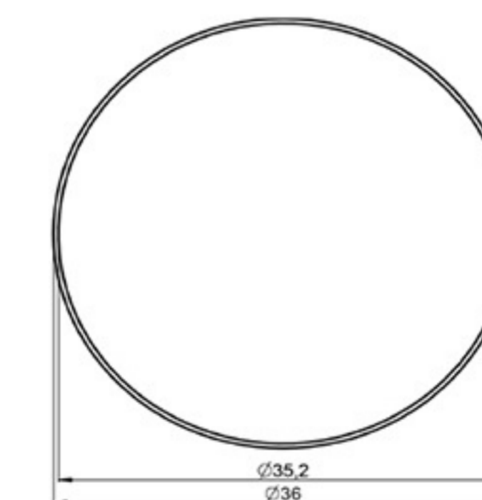
DUST-PROOF PROFILE
