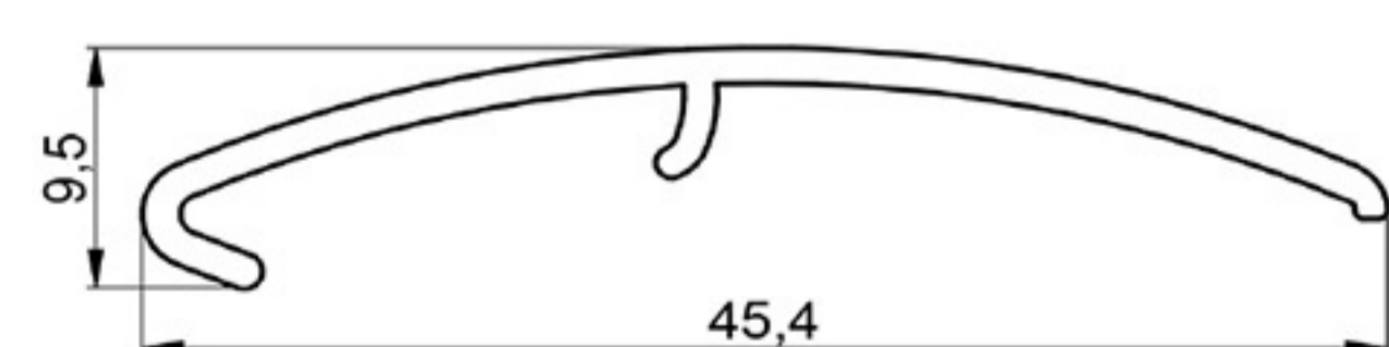
LIGHTING COVER PROFILE
