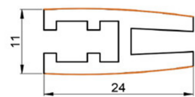
PROFILE FOR PARTITIONS
