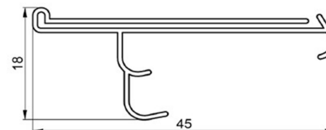
PARTITIONS CONNECTOR
