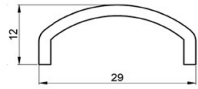
PROFILE FOR PARTITIONS
