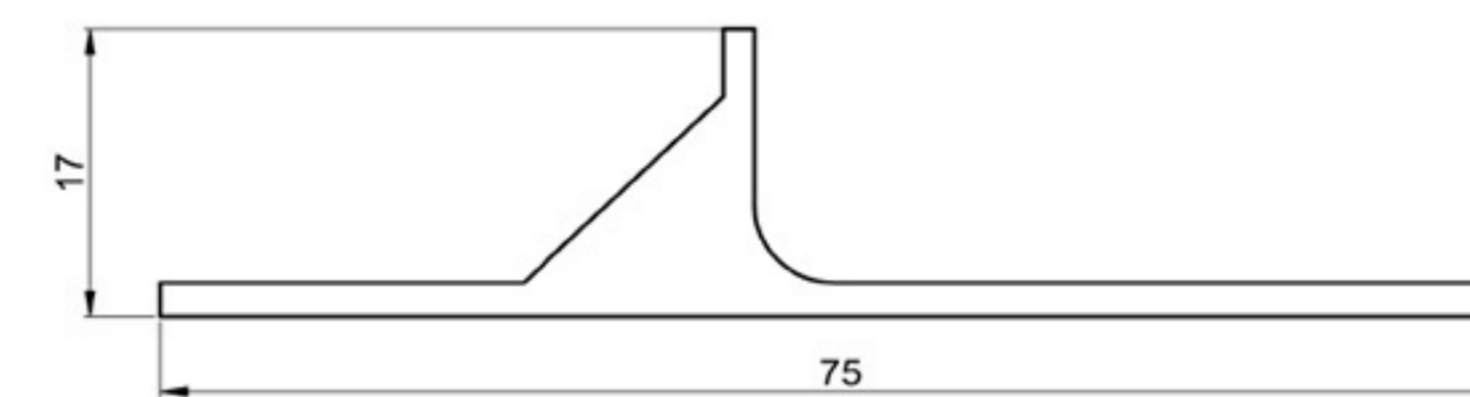
SKIRTING PROFILE
