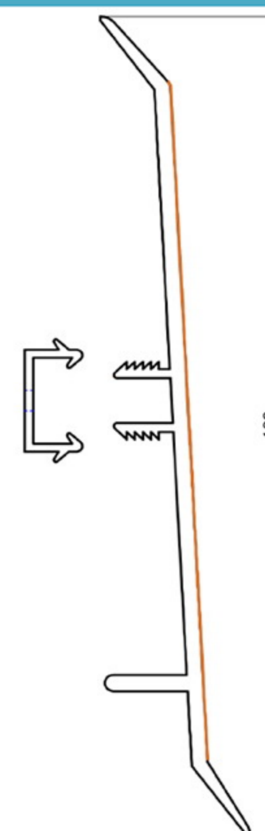
INSERTING DECO PROFILE
