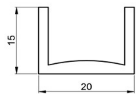
PANEL FRAME
