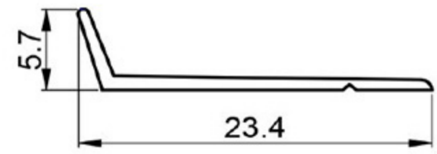
GUIDE RAIL PROFILE
