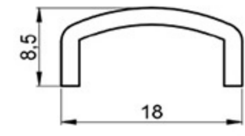
FRAME PROFILE
