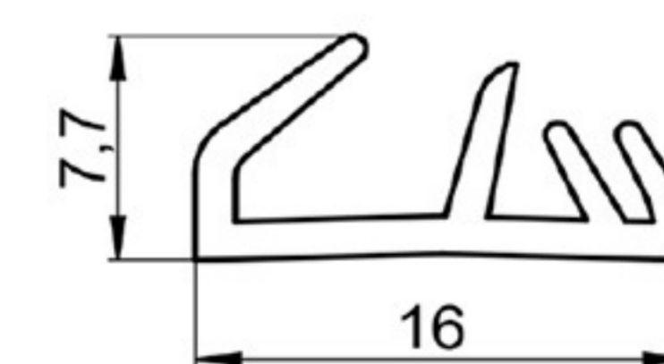
DECO PANELS SPACER
